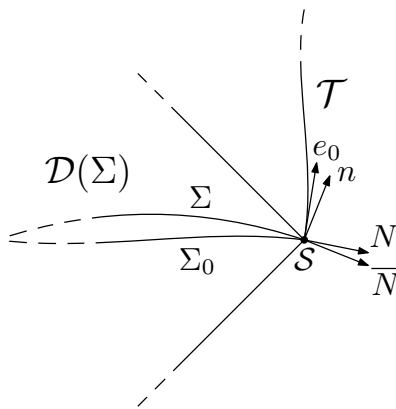
Figure 2: The classical solution in the domain of dependence \mathcal{D}(\Sigma) .
