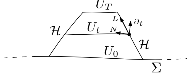
Figure 1: Local domain of dependence.
