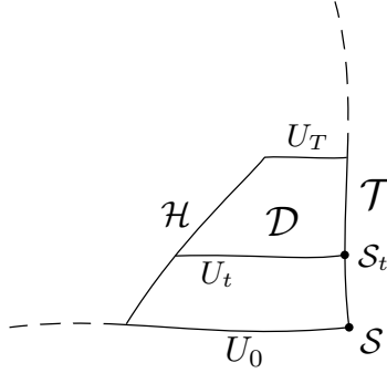
Figure 3: A local domain of dependence region near the boundary.
