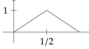
FIGURE 2. The graph of the function \phi .
