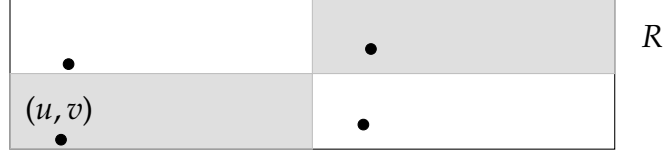
FIGURE 3. The quadruple Q .
