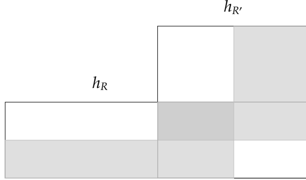
FIGURE 1. Two Haar functions.
